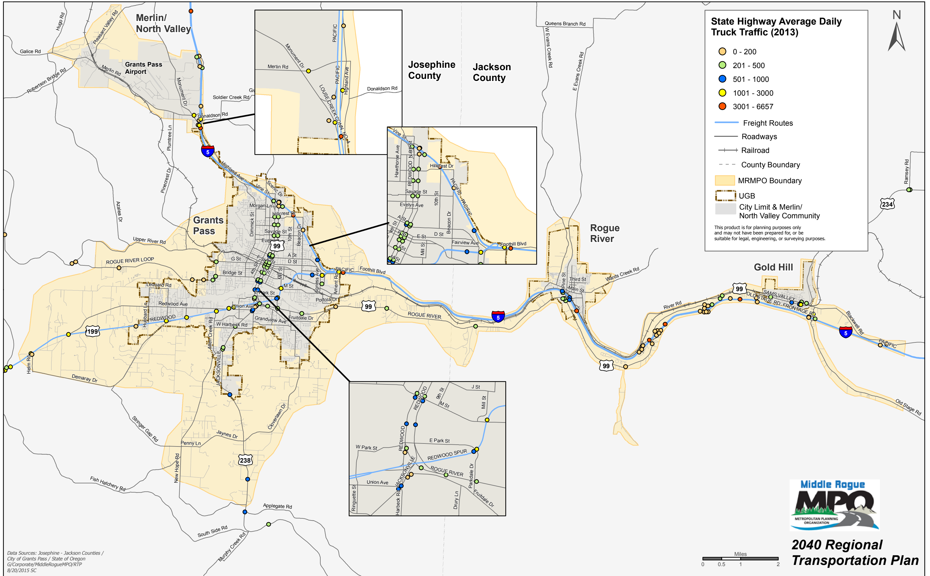
Map 5-5 - State Highway Average Daily Truck Traffic
